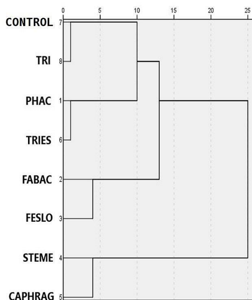
Figure 3. Dendrogram – cluster analysis (biological data from both depth and sampling date), between groups-method (IBM-SPSS)
